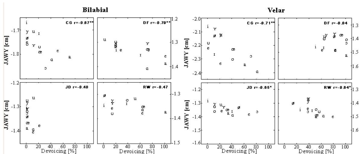
Figure 3: Scatterplots of the percentage of devoicing and the vertical jaw position at consonant onset of bilabials (left) and velars (right) for means of each speaker.
