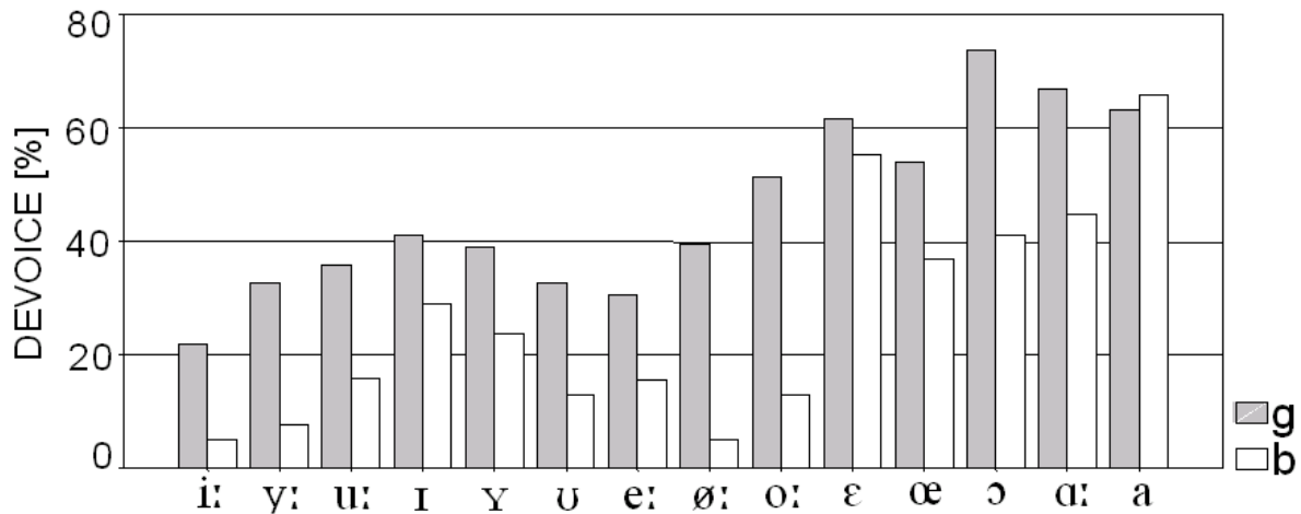
Figure 2: Percentage of devoicing, shown for each vowel and the contexts /b/ and /g/. The vowels are ordered by their phonological vowel height. Mean values are 46.3 per cent for the velar and 26.4 per cent for the bilabial.
