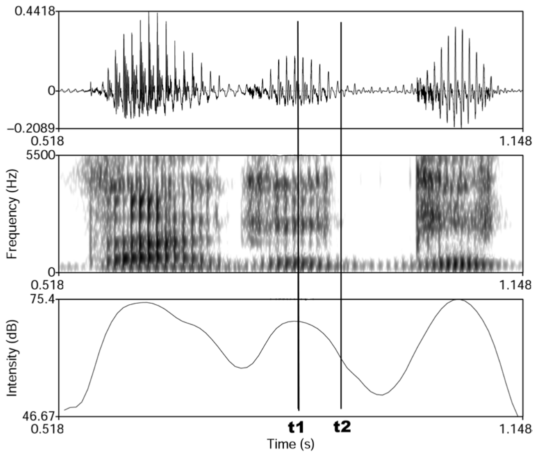
Figure 1: Procedure for acoustic labelling: Shown is: in the upper panel the oscillogram, in the middle panel the spectrogram and in the lower panel the intensity contour. The left black bar (t1) indicates the landmark of the maximal intensity of the vowel. The right bar (2) indicates the 6dB intensity decrease measured from the point of maximal intensity.
